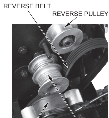
FORWARD BELT
